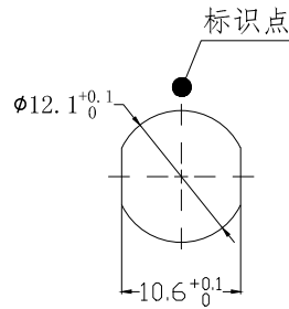
Panel cut-outs 建议安装开孔尺寸
