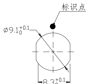
Panel cut-outs 建议安装开孔尺寸
