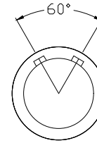
Socket front view 插座前视图
