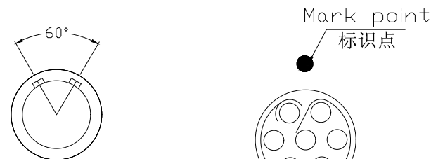
Plug front view 插头前视图
