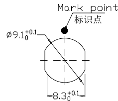
Panel cut-outs 建议安装开孔尺寸
