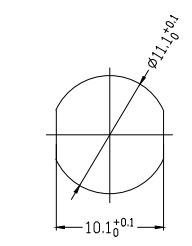
Panel cut-outs 建议安装开孔尺寸
