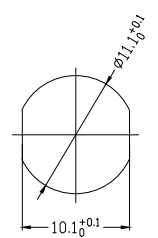
Panel cut-outs 建议安装开孔尺寸
