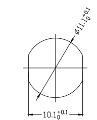
Panel cut-outs 建议安装开孔尺寸
