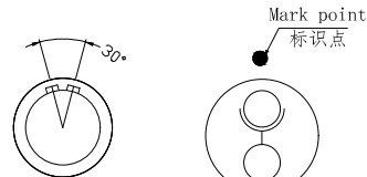
Plug front view 插头前视图
