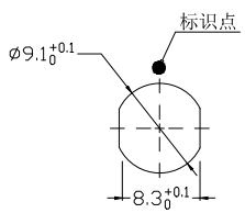
Panel cut-outs 建议安装开孔尺寸
