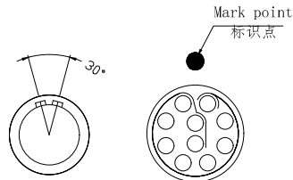
Socket front view 插座前视图 view K K向孔位排列
