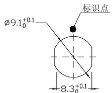
Panel cut-outs 建议安装开孔尺寸
