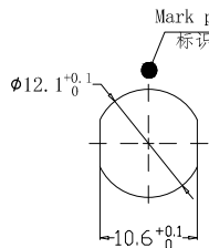
Panel cut-outs 建议安装开孔尺寸
