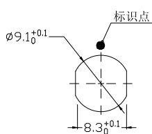
Panel cut-outs 建议安装开孔尺寸
