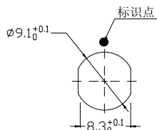
Panel cut-outs 建议安装开孔尺寸
