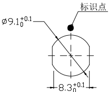
Panel cut-outs 建议安装开孔尺寸
