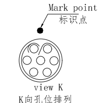
Plug front view 插头前视图
