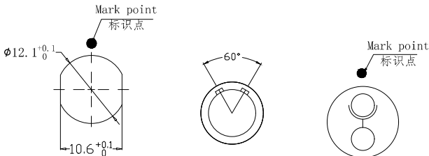
Panel cut-outs 建议安装开孔尺寸
