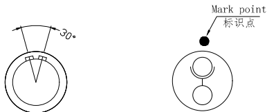
Socket front view 插座前视图
