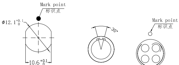
Panel cut-outs 建议安装开孔尺寸 Socket front view 插座前视图 view K K向孔位排列
