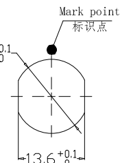
Panel cut-outs 建议安装开孔尺寸
