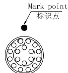
view K K到孔位排列
