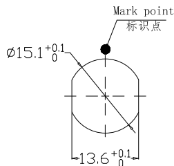
Panel cut-outs
