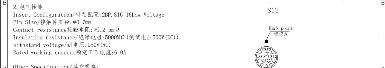
view K K向孔位排列
