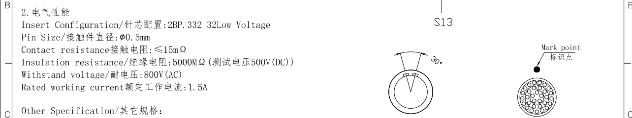
Socket front view 插座前视图
