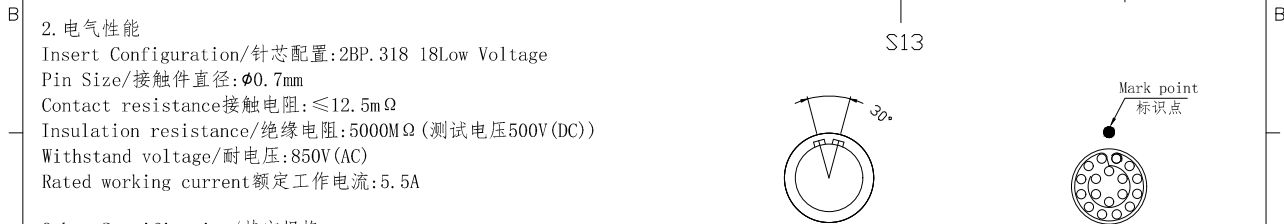
Socket front view 插座前视图
