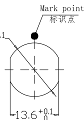
Panel cut-outs 建议安装开孔尺寸
