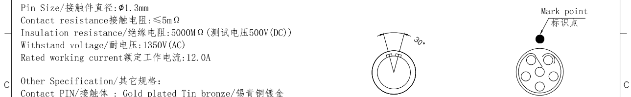
Socket front view 插座前视图
