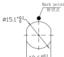
Panel cut-outs 建议安装开孔尺寸
