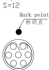
view K K向孔位排列
