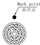
view K K孔孔位排列
