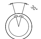
Socket front view 插座前视图
