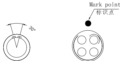
Socket front view 插座前视图
