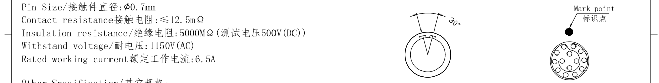
Socket front view 插座前视图
