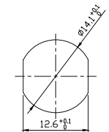
Panel cut-outs 建议安装开孔尺寸
