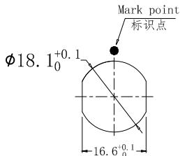
Panel cut-outs 建议安装开孔尺寸
