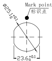
Panel cut-outs 建议安装开孔尺寸
