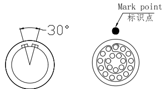
Socket front view 插座前视图
