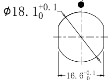
Panel cut-outs 建议安装开孔尺寸
