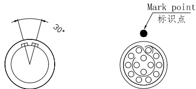
Socket front view 插座前视图
