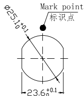
Panel cut-outs 建议安装开孔尺寸
