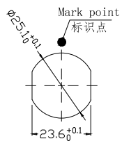
Panel cut-outs 建议安装开孔尺寸
