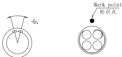
Socket front view 插座前视图
