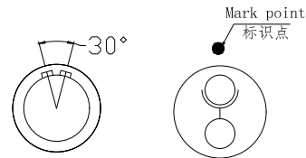
Socket front view 插座前视图
