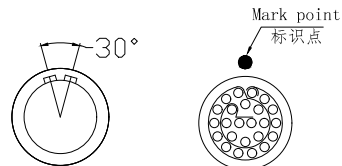
Socket front view 插座前视图
