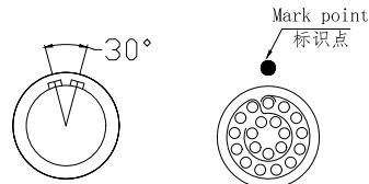
Socket front view 插座前视图
