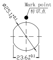
Panel cut-outs 建议安装开孔尺寸
