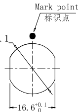
Panel cut-outs 建议安装开孔尺寸
