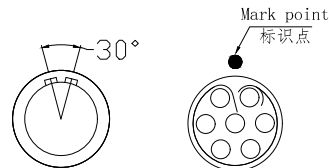
Socket front view 插座前视图
