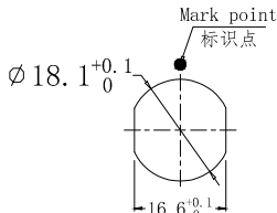
Panel cut-outs 建议安装开孔尺寸
